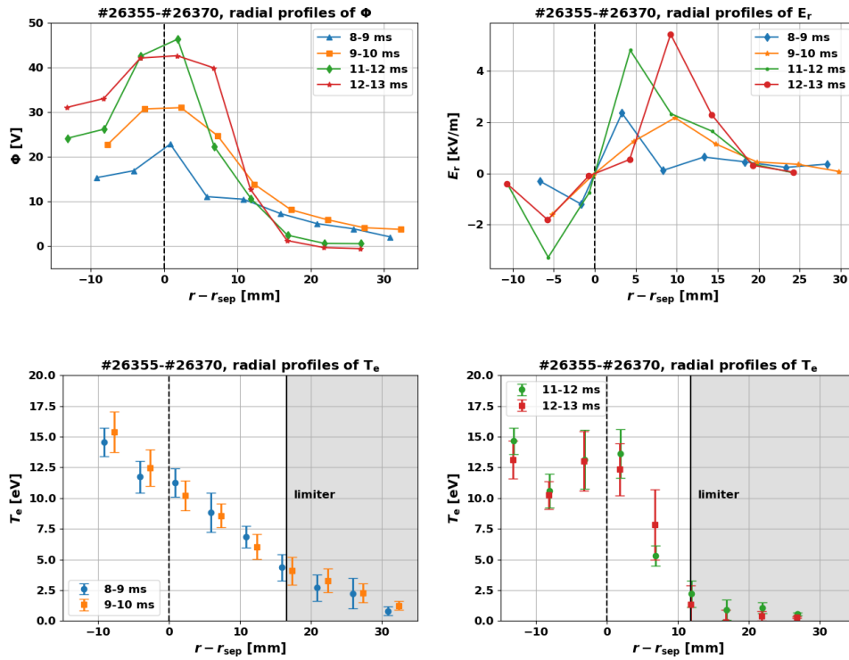
Figure 4: Radial profiles of plasma potential, radial electric field and electron temperature.
