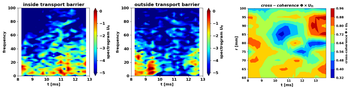
Figure 6: Spectrogram of the floating potential (left), cross-coherence between plasma and floating potentials (right).
