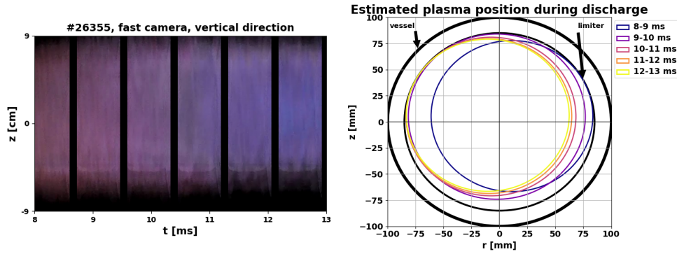
Figure 5: Plasma position determined by fast camera (left), and by Mirnov coils (right).
