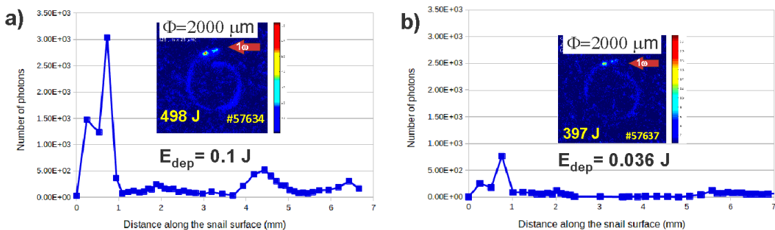
Fig.5: Results of Cu K \alpha - measurements illustrating the effect of the laser beam with linear (a) and circular (b) polarization on the energy deposited by HE along the surface of a target with a diameter of 2000 \mu\text{m} .
