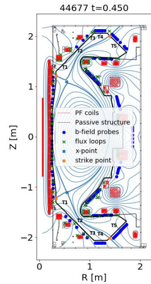
Figure 1 The location of magnetics used in EFIT++ and poloidal flux for shot 44677 at t=0.5 s
