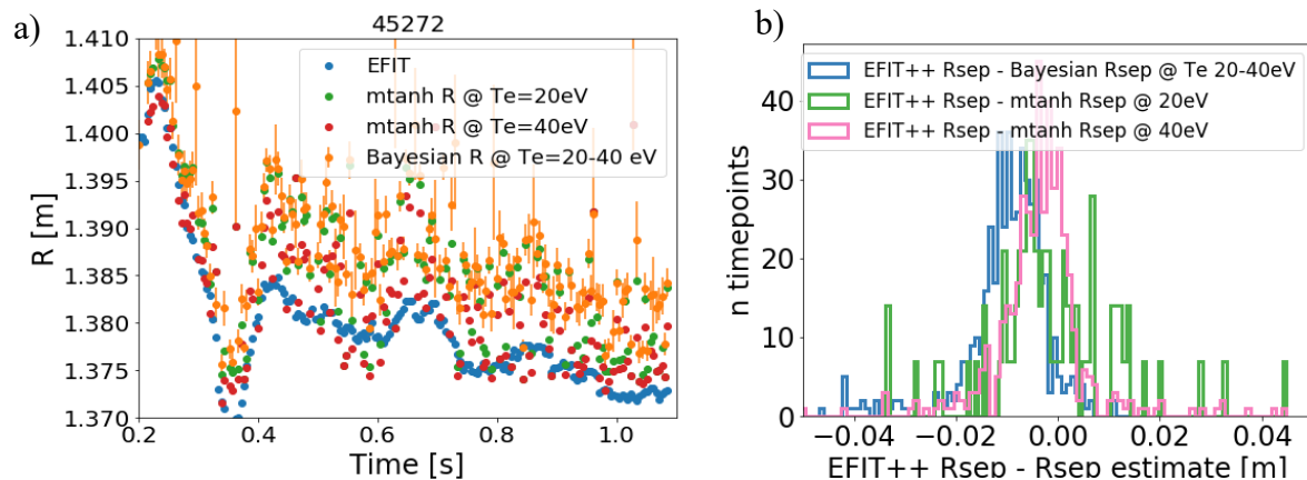
Figure 4 The LCFS location at z=0.015\text{m} (the TS line of sight) from EFIT++ compared to R at T_e = 20, 40\text{eV} from \text{mtanh} fits to the TS profiles, and the LCFS from the Bayesian analysis for a) an example shot 45272 vs time for inter-ELM times and b) the difference in LCFS across a range of shots and H-mode times.
