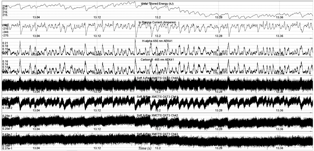
(a). Time slice of fluctuations before the gyrotron dropout at 15 seconds, showing typical high iota quasi-continuous oscillatory behavior [4], although there are unusual occasional small “sawteeth” (perhaps due to very clean wall conditions and low neutral pressure).
