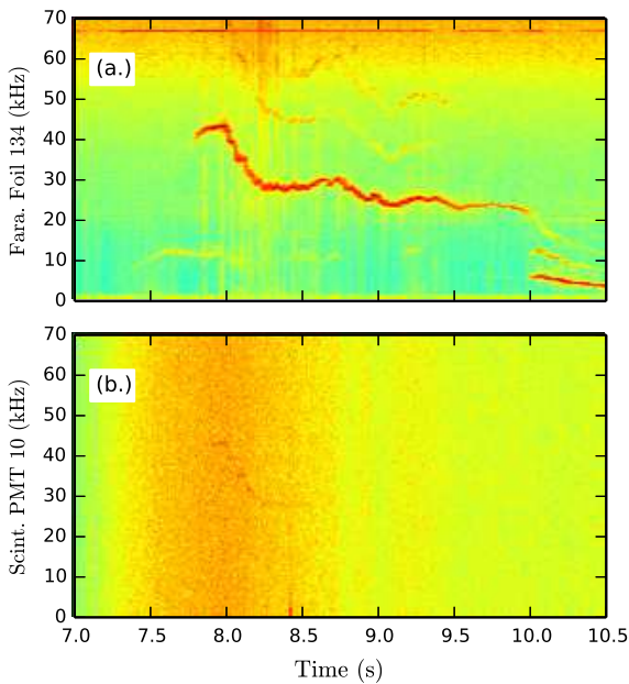
Figure 3: A spectrogram from Faraday foil 134, (a.), and a spectrogram from scintillator PMT 10, (b.) showing coherent n=2 mode losses.
