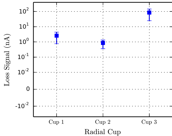
Figure 6: Integrated fast ion loss signal as a function of radial position for the Faraday cups closest to the midplane poloidally. Cup 1 is closest to the plasma while cup 3 is closest to the wall (2.5 cm between cups).
