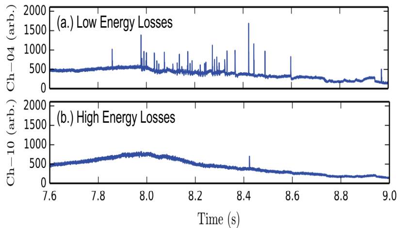
Figure 4: ELM induced losses in the scintillator probe present in the low energy PMT channel 4 and absent in the high energy PMT channel 10.
